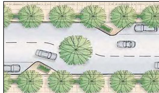
Figure 4 - Chicane
