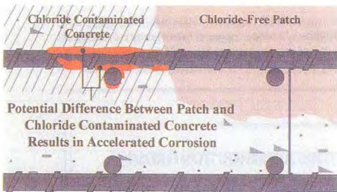
"Ring Anode" Corrosion (without Galvashield XP)
