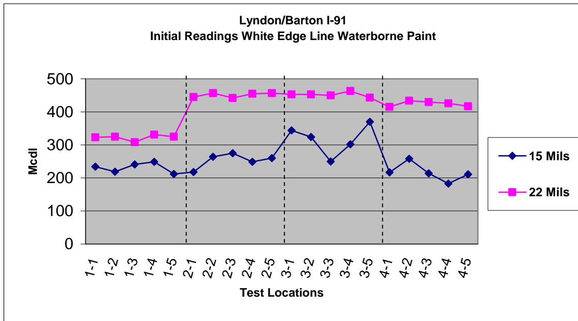
Figure 11- Initial Readings on White Paint, I-91 Lyndon/Barton
