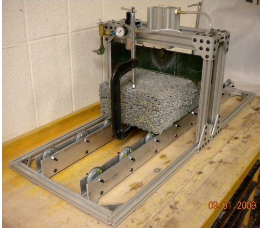
Figure 5.4: Plow Modeling Apparatus in Use
