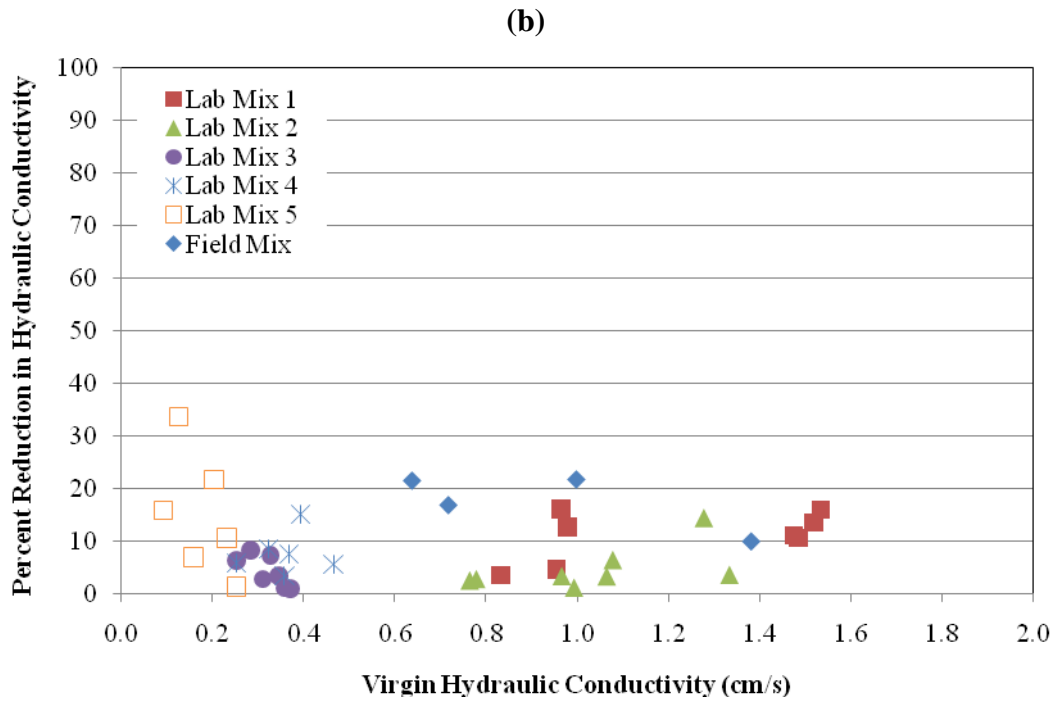
Figure 4.6: Changes in Hydraulic Conductivity after Vacuuming
