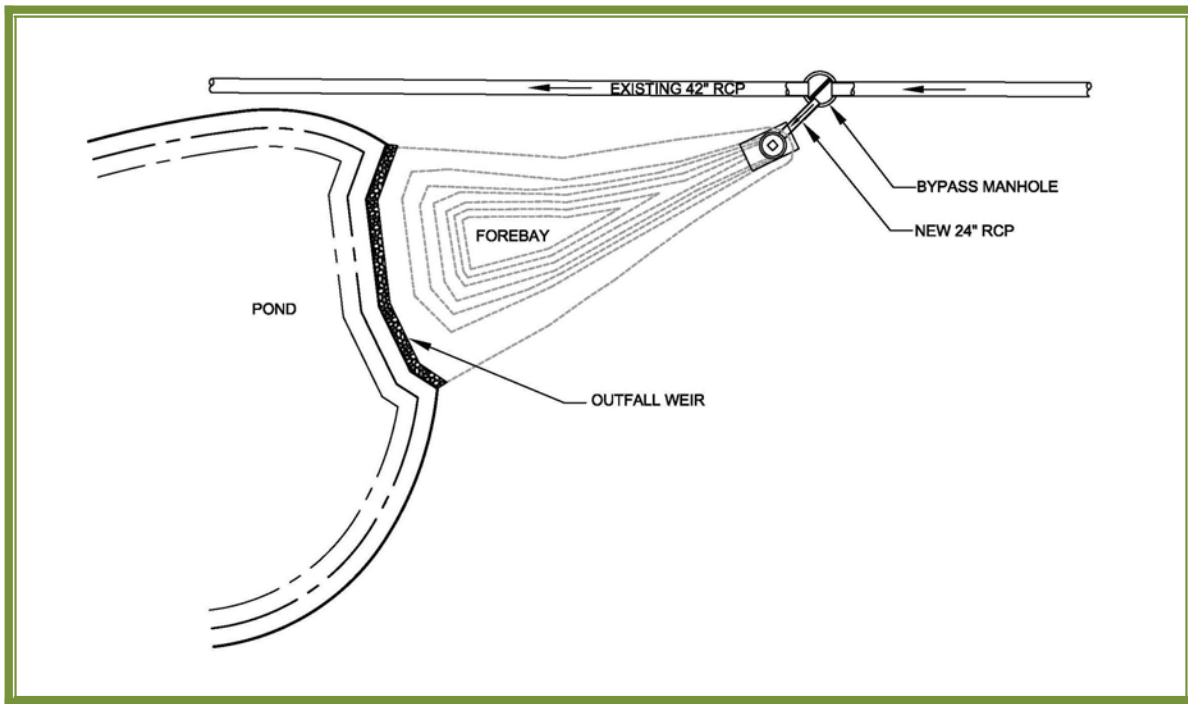
Forebay with Forced Hydraulic Jump – Plan View
