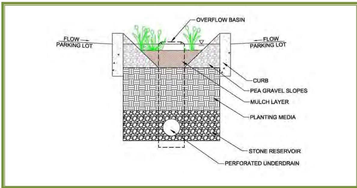
Micro-bioretention section detail (MDE, 2008)
