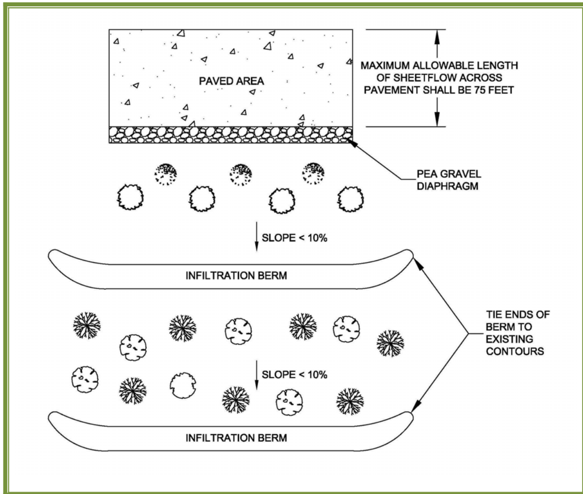
Infiltration berm plan view (CWP, 2009)
