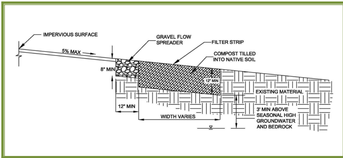
Compost-amended vegetated filter strip cross section (adapted from WSDOT, 2008)
