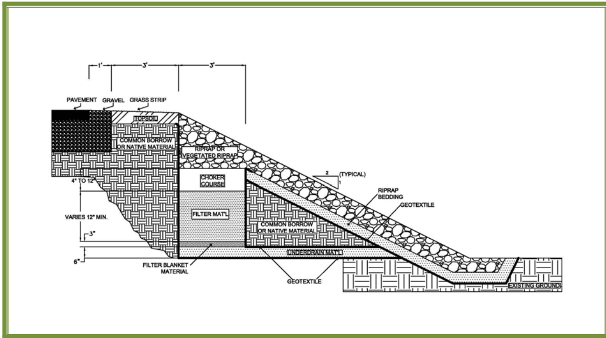
Embankment media filter with day-lighted drainage layer (CEI)
