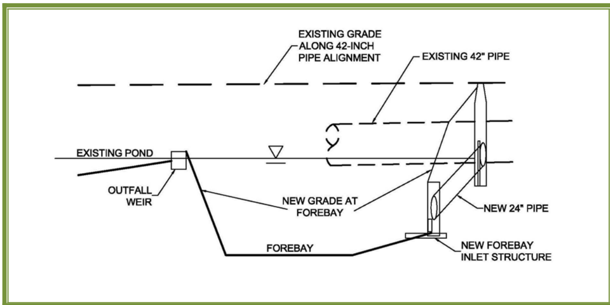
Forebay with Forced Hydraulic Jump – Profile
