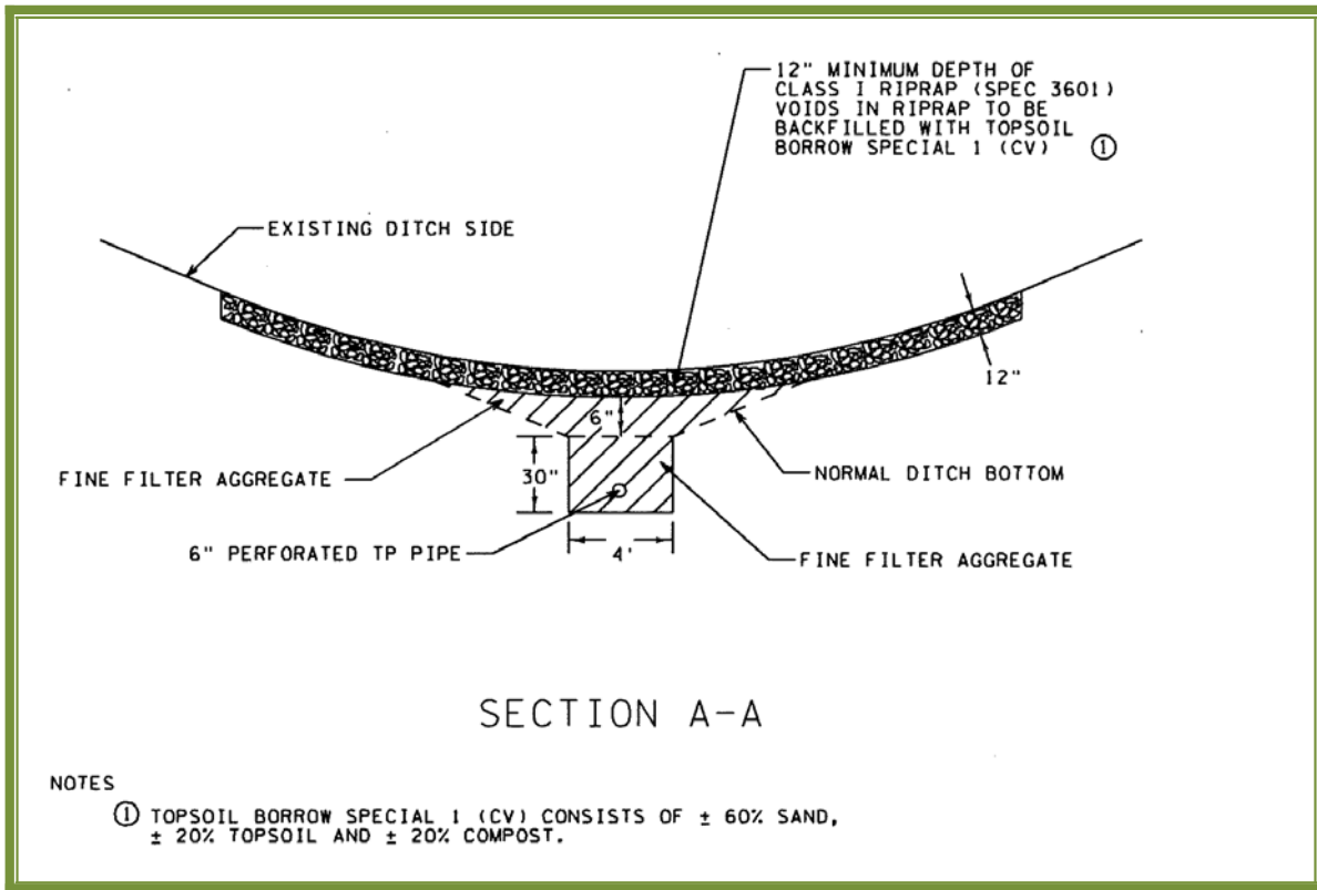
Minnesota Permeable Ditch Block: section (Irish, 2011)
