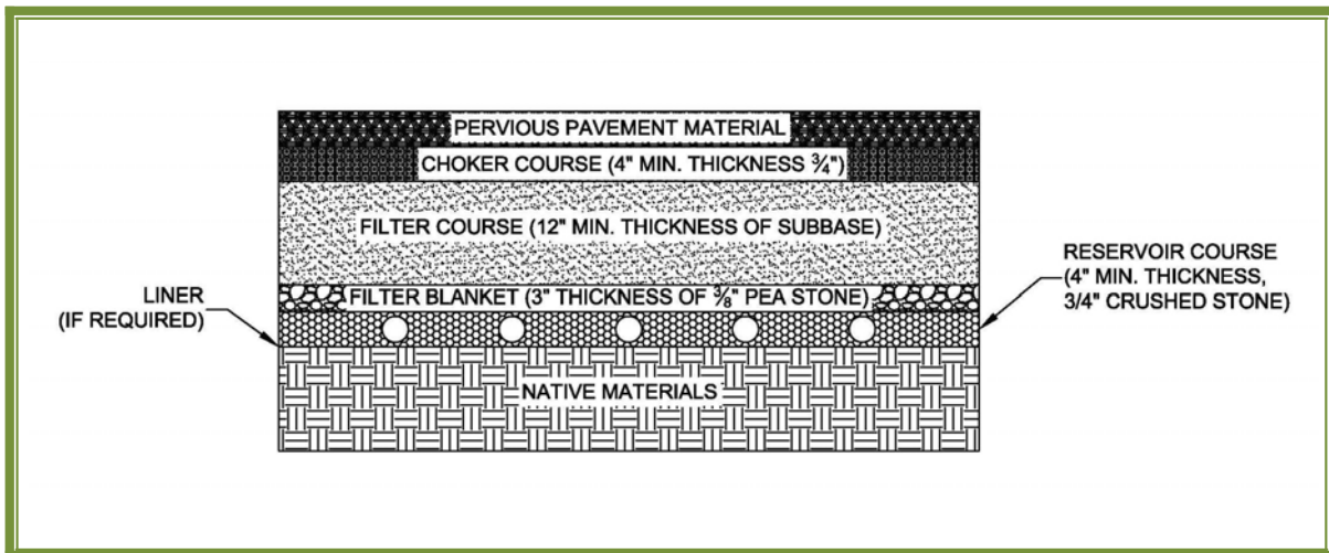
Typical section of pervious pavement (porous asphalt or concrete), underdrained (adapted from the University of New Hampshire Stormwater Center)
