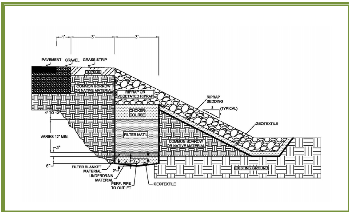
Embankment media filter with underdrain (CEI)
