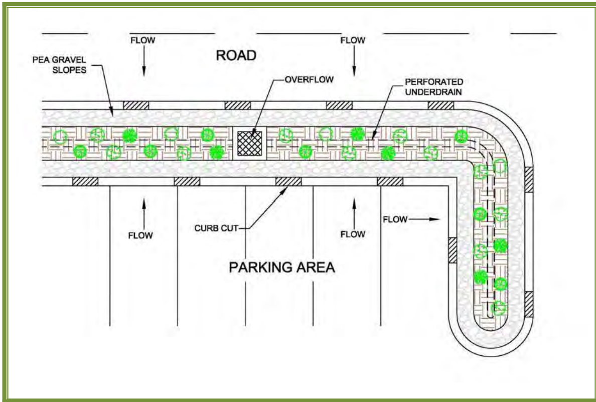
Micro-bioretention plan view (MDE, 2008)
