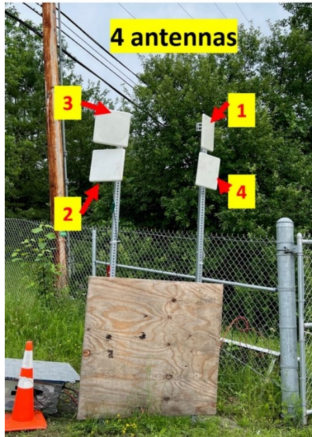
Fig. 22: 4-channel configuration
