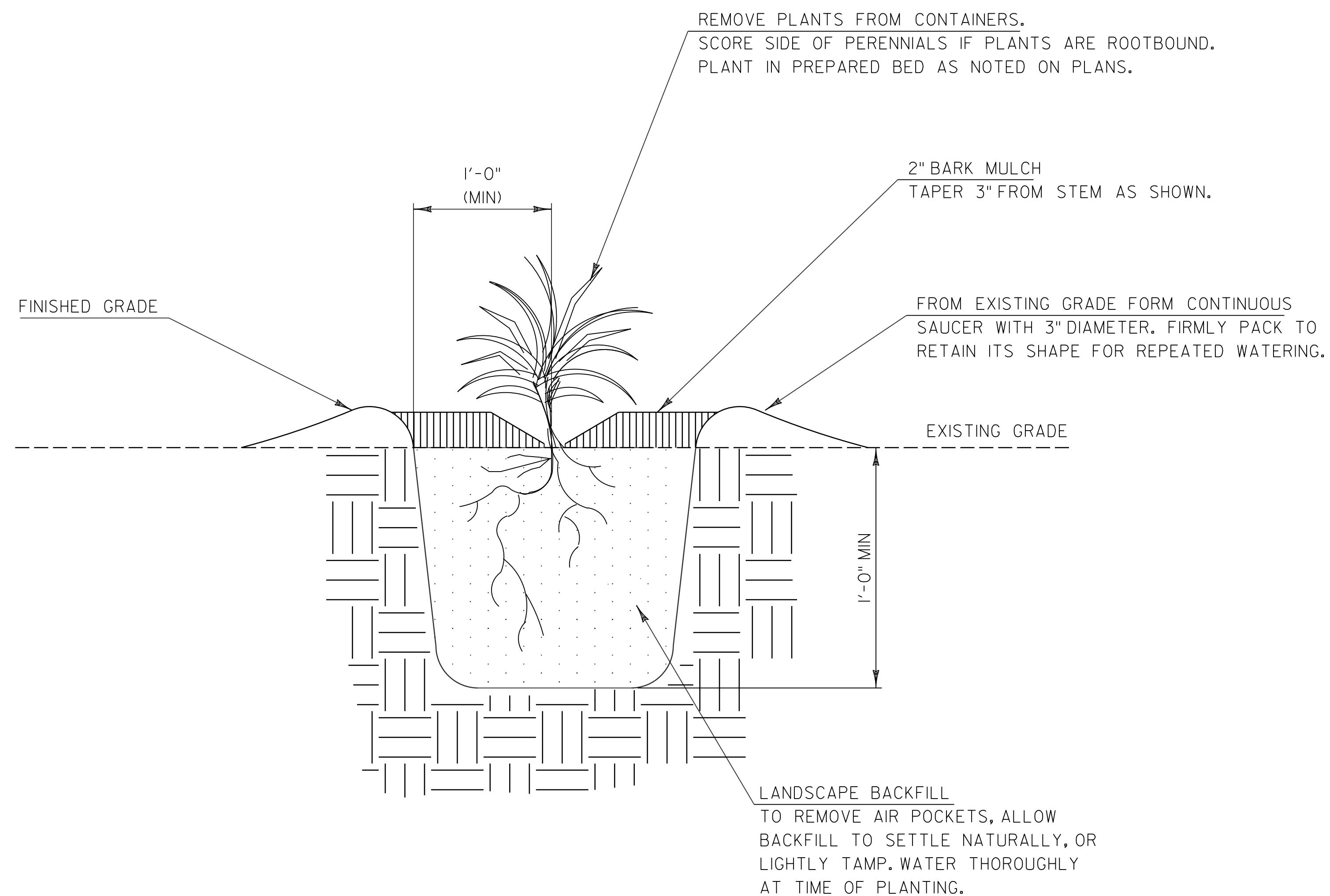
PERENNIAL, GROUND COVER AND VINES PLANTING DETAIL
