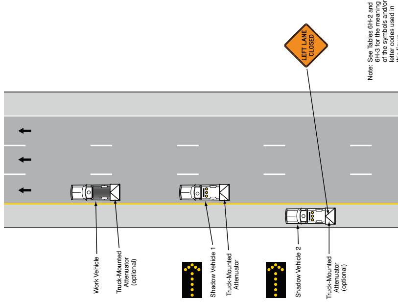
Typical Application 35
